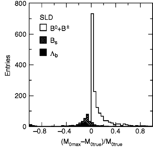
FIG. 2. The relative deviation of the maximum missing mass from the true missing mass for simulated B hadron decays; the contributions from different B species are indicated separately: B^0 and B^\pm (open), B_s^0 (cross-hatched), and \Lambda_b (dark shaded).
